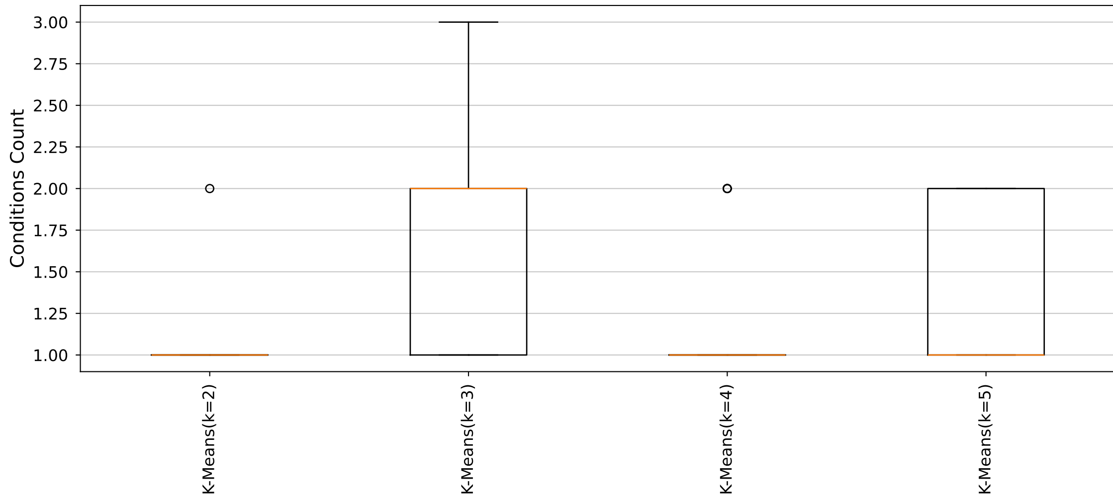
YARA Rules Conditions Count Distribution (Cluster38_Size5 dataset)
